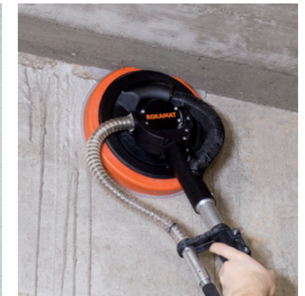
Grinding concrete burrs
